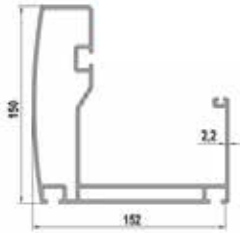
Outstanding Serie Front Gutter - 4,398 kg / m 152mm x 150mm
