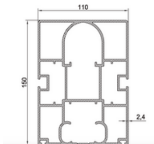
Outstanding Serie Guide Rail - 7,168kg / m 110mm x 150mm
