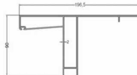
Motor Top Cover
